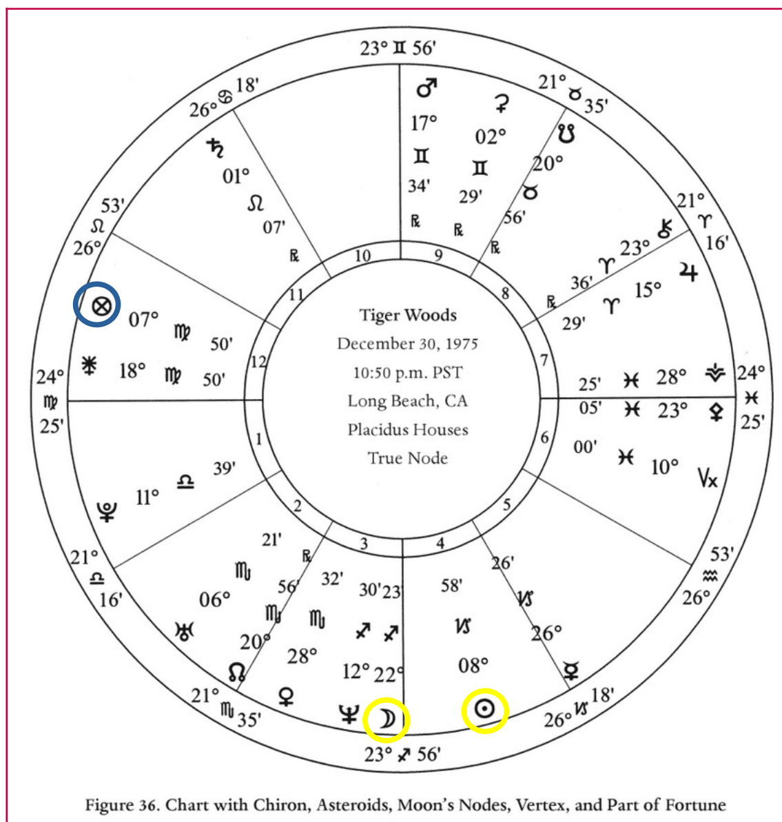
Figure 3. Riske (2010: 298) In this font also the symbols \otimes , \odot and \rangle are the same size.
